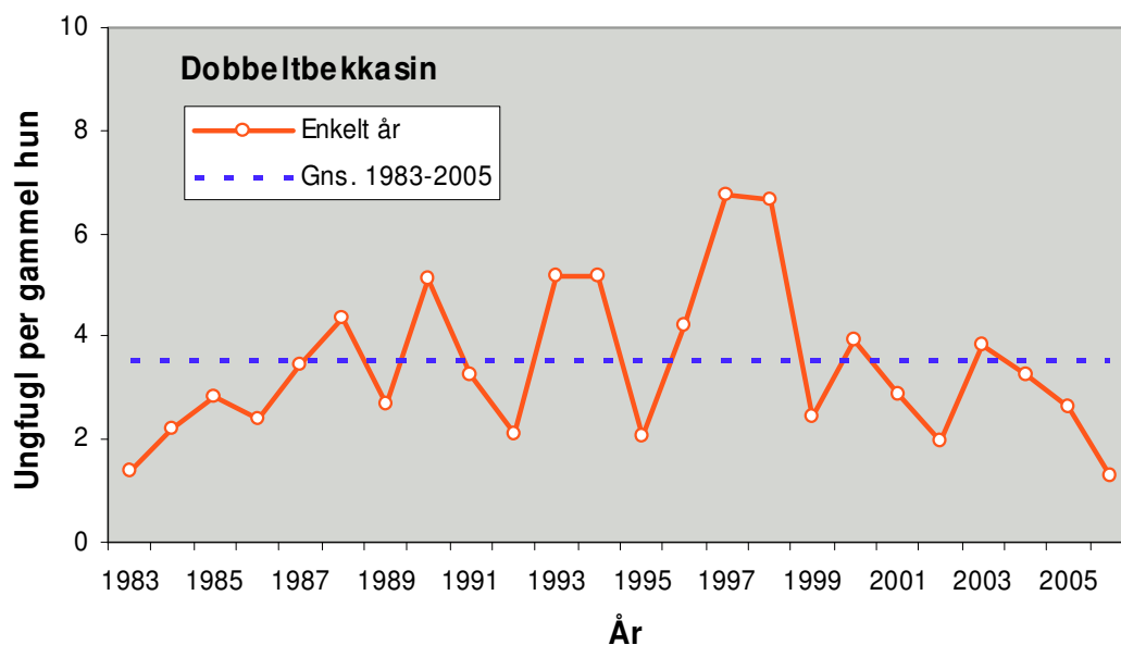
Figur 5. Ynglesucces for dobbeltbekkasin, udtrykt som antal ungfugle per gammel hun i de indsendte vinger fra jagtsæsonerne 1983/84-2006/07. Reproductive success of Snipe expressed as the number of juveniles per adult female of received wings from the hunting seasons 1983/84-2006/07.
