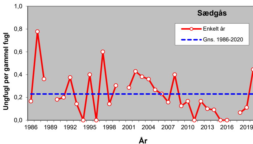
Figur 5. Ynglesucces for sædgås, udtrykt som antal ungfugle per gammel fugl i de indsendte vinger fra jagtsæsonerne 1986/87-2020/21. Reproductive success of Bean Goose expressed as the number of juveniles per adult of received wings from the hunting seasons 1986/87-2020/21.
