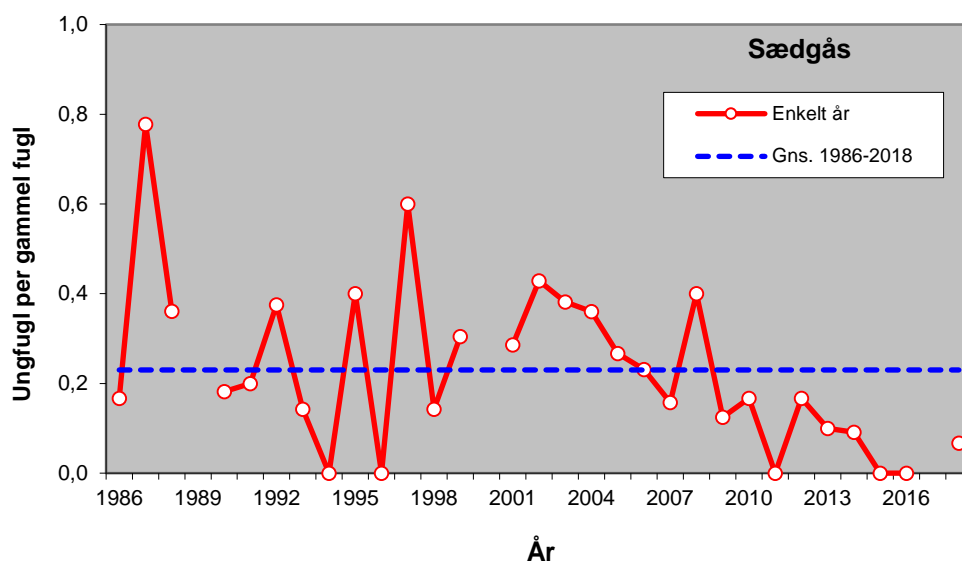
Figur 5. Ynglesucces for sædgås, udtrykt som antal ungfugle per gammel fugl i de indsendte vinger fra jagtsæsonerne 1986/87-2018/19. Reproductive success of Bean Goose expressed as the number of juveniles per adult of received wings from the hunting seasons 1986/87-2018/19.
