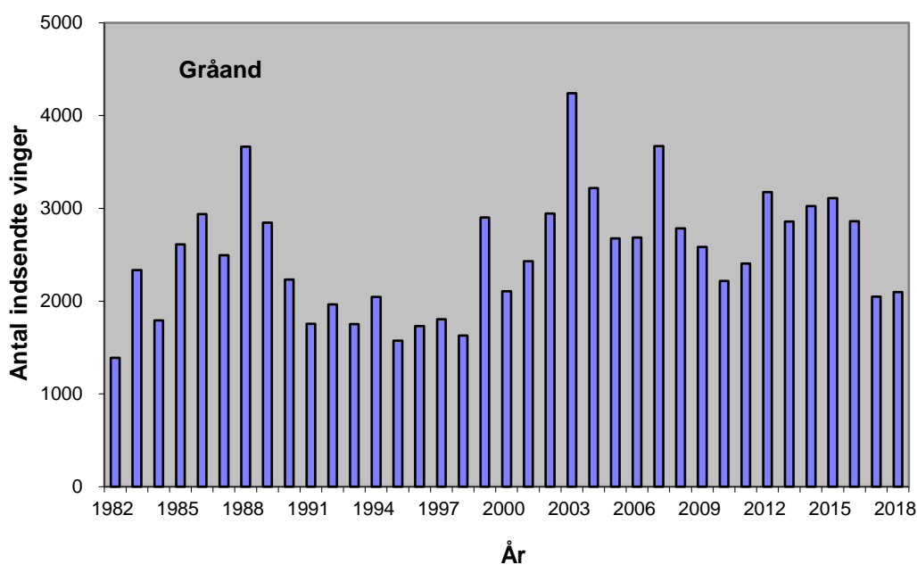
Figur 2. Antallet af indsendte vinger af gråand fra jagtsæsonerne 1982/83-2018/19. The number of Mallard wings received from the hunting seasons 1982/83-2018/19.
