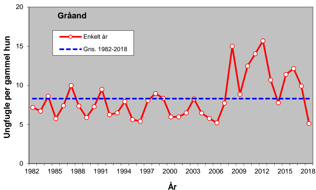
Figur 5. Ynglesucces for gråand, udtrykt som antal ungfugle per gammel hun i de indsendte vinger fra jagtsæsonerne 1982/83-2018/19. Reproductive success of Mallard expressed as the number of juveniles per adult female of received wings from the hunting seasons 1982/83-2018/19.
